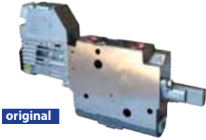
Hydraulic Valve Section New Holland T6s TSA's Case Maxxum MXU Puma - Electronic Operation - Cable Type - 43631
